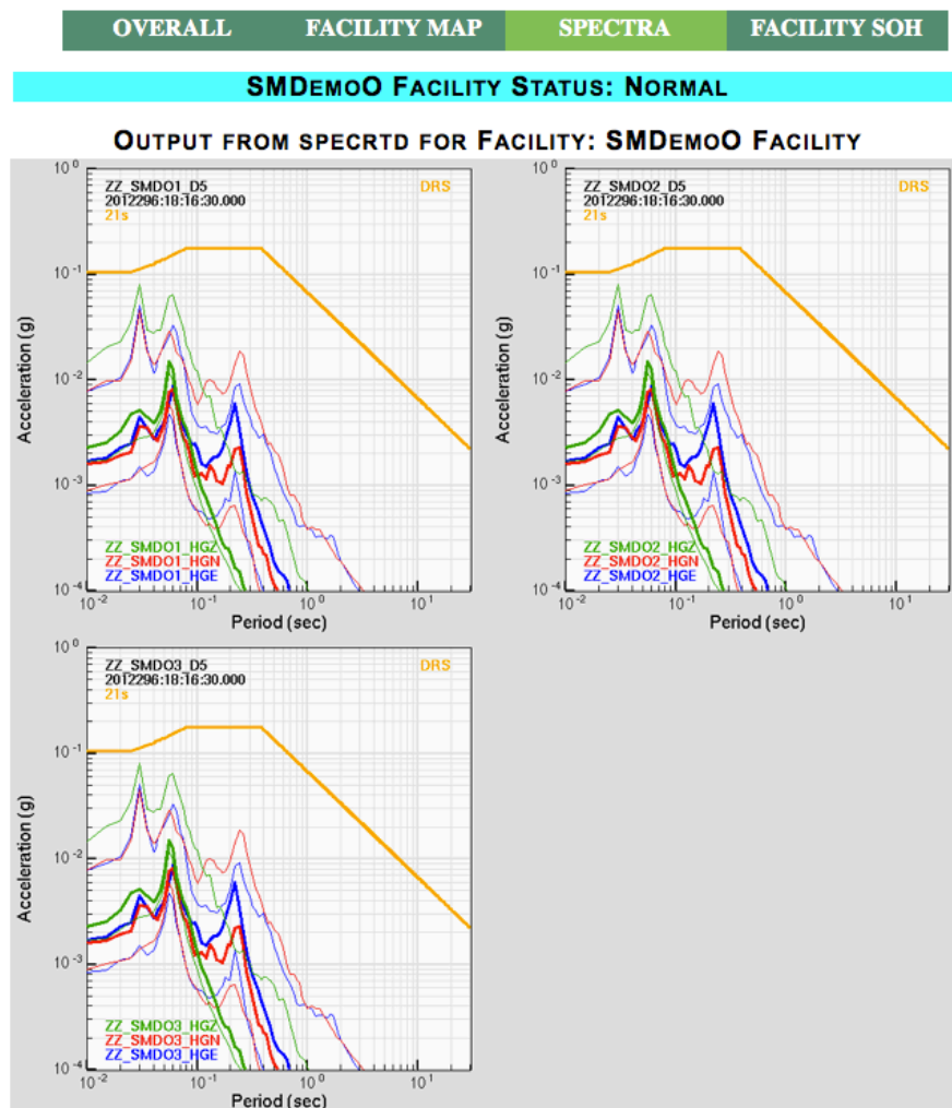
Figure 4. Bighorn web display: snapshot of real-time spectral calculations
