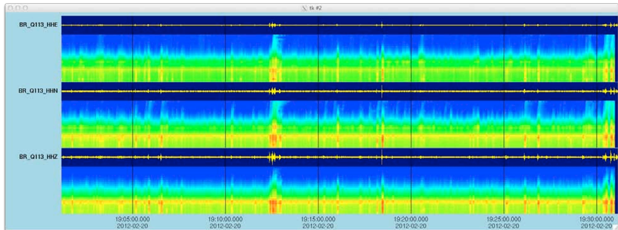
Figure 2. Display of real-time max PSA as color-mapped frequency-slices below acceleration data for three channels.
