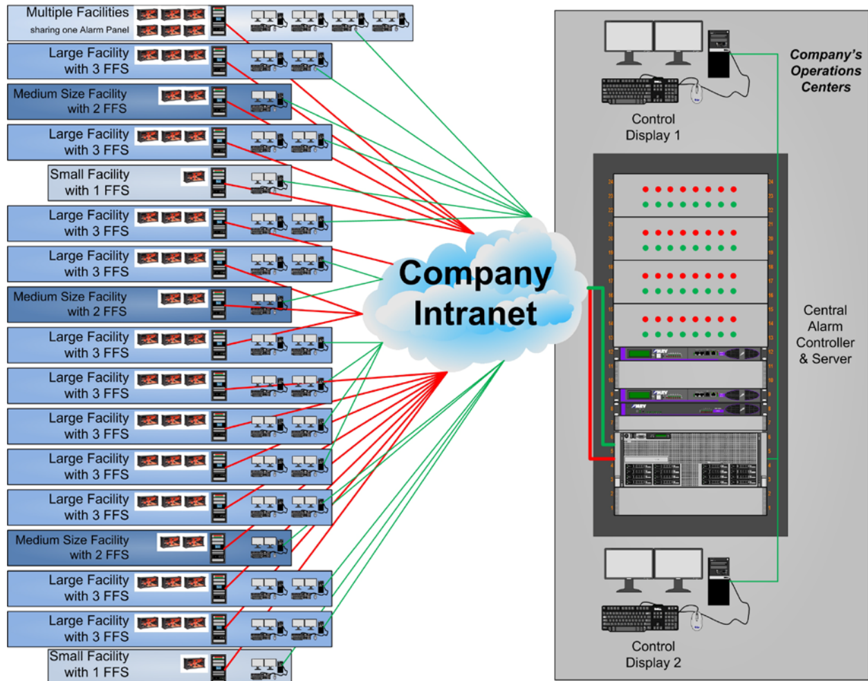
Figure 8. Schematic of system network.
