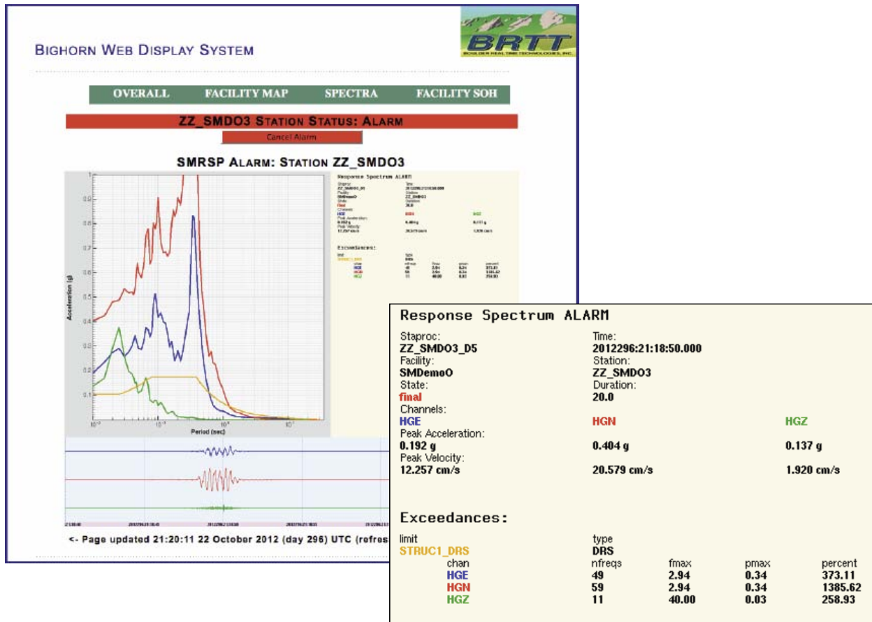
Figure 6. Bighorn web display: event report with zoomed in insert
