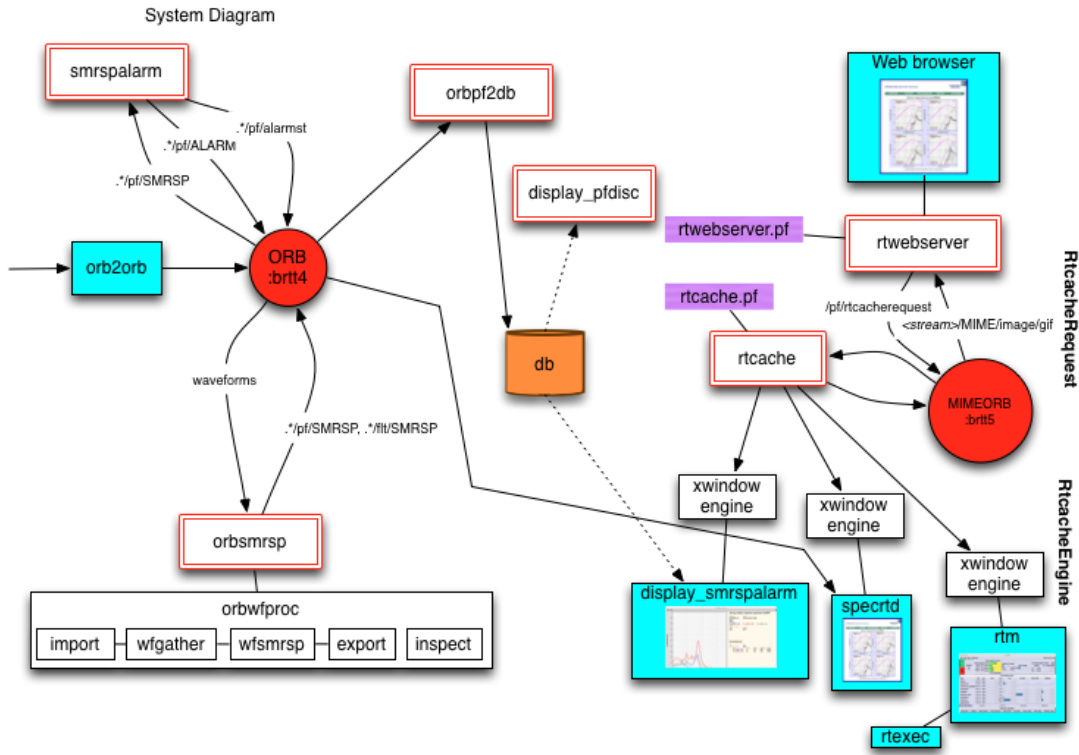
Figure 1. Bighorn layout information flow diagram
